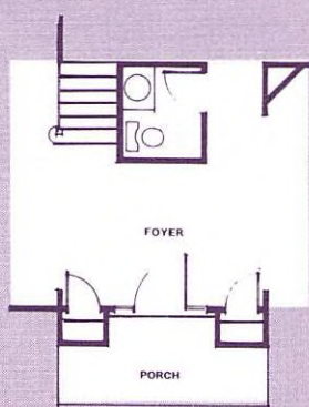
FOYER PLAN FOR B & C ELEVATION
